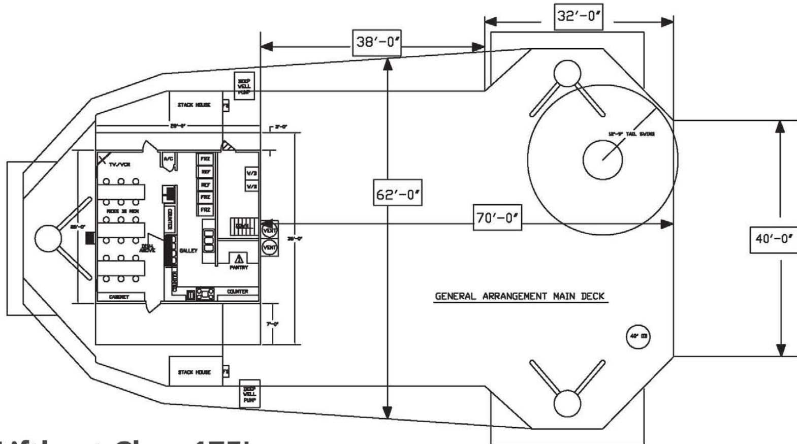
Liftboat Class 175' M/V Ram XVI and M/V Ram XVII
