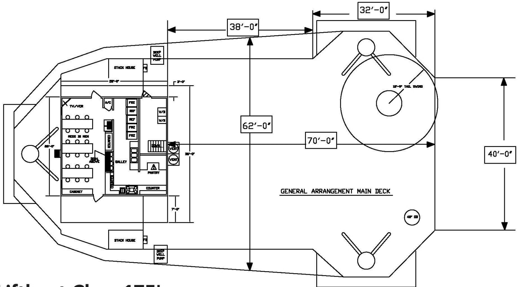
Liftboat Class 175' M/V Ram XVII
